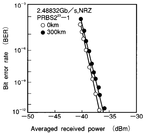
Fig.5 BER characteristics
