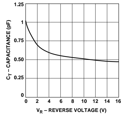
Figure 15. Total Capacitance vs. Reverse Voltage—HSMS-2810 Series.
