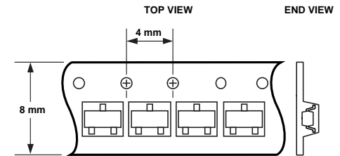
Figure 17. Options -TR1, -TR2 for SOT-23 Packages.
