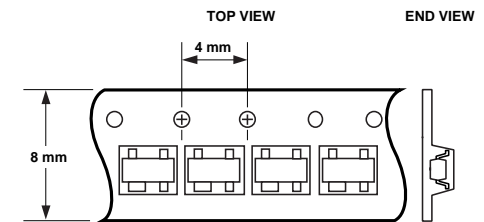
Figure 18. Options -TR1, -TR2 for SOT-143 Packages.
