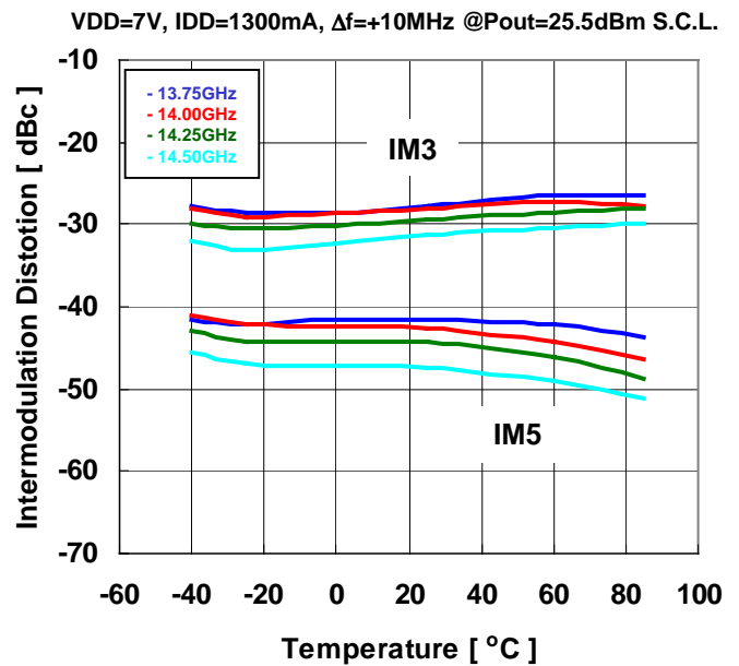
IMD PERFORMANCE vs. TEMPERATURE
