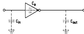
Figure 11. Parasitic Capacitances of the Amplifier
