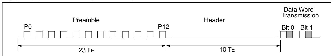
FIGURE 8-3: PREAMBLE/HEADER FORMAT
