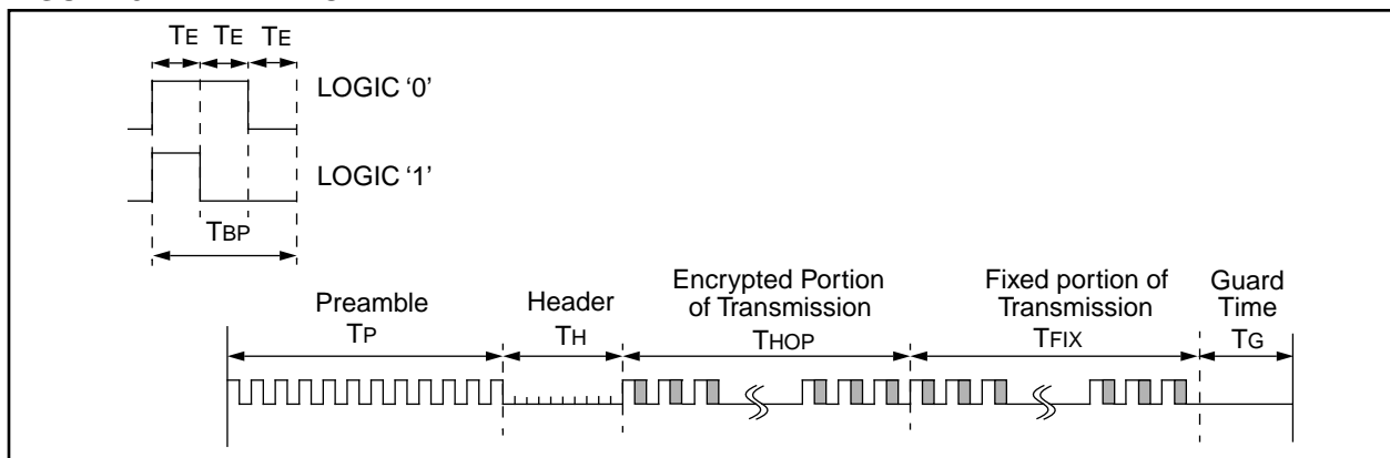
FIGURE 8-3: PREAMBLE/HEADER FORMAT
