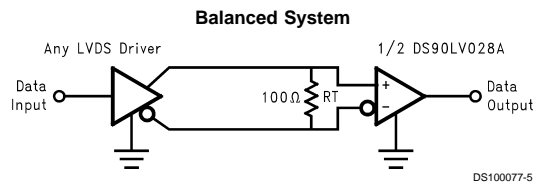
FIGURE 3. Point-to-Point Application
