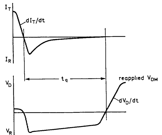
Fig. 2b Circuit-commutated turn-off time definition.
