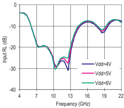
Figure 10. Input Return Loss and Voltage
