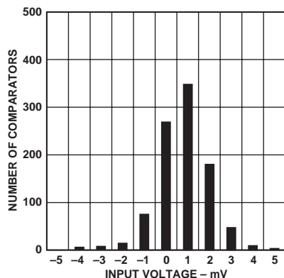
Figure 2. Typical Distribution of Input Offset Voltage
