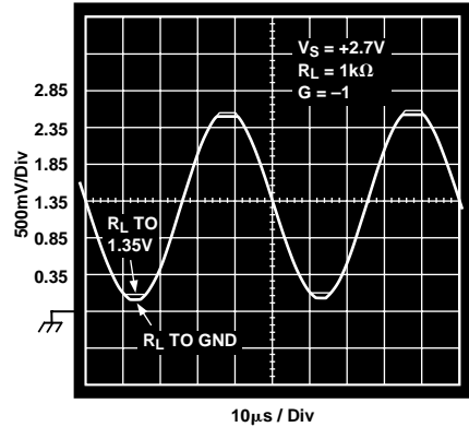
Figure 35. Output Swing
