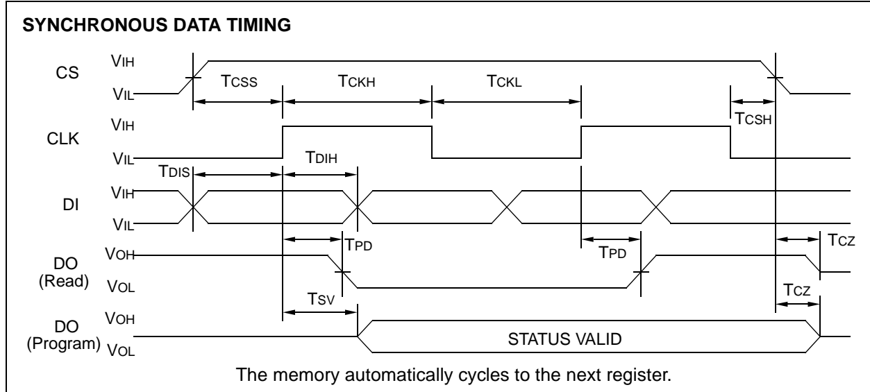
FIGURE 4-1: TIMING DIAGRAMS
